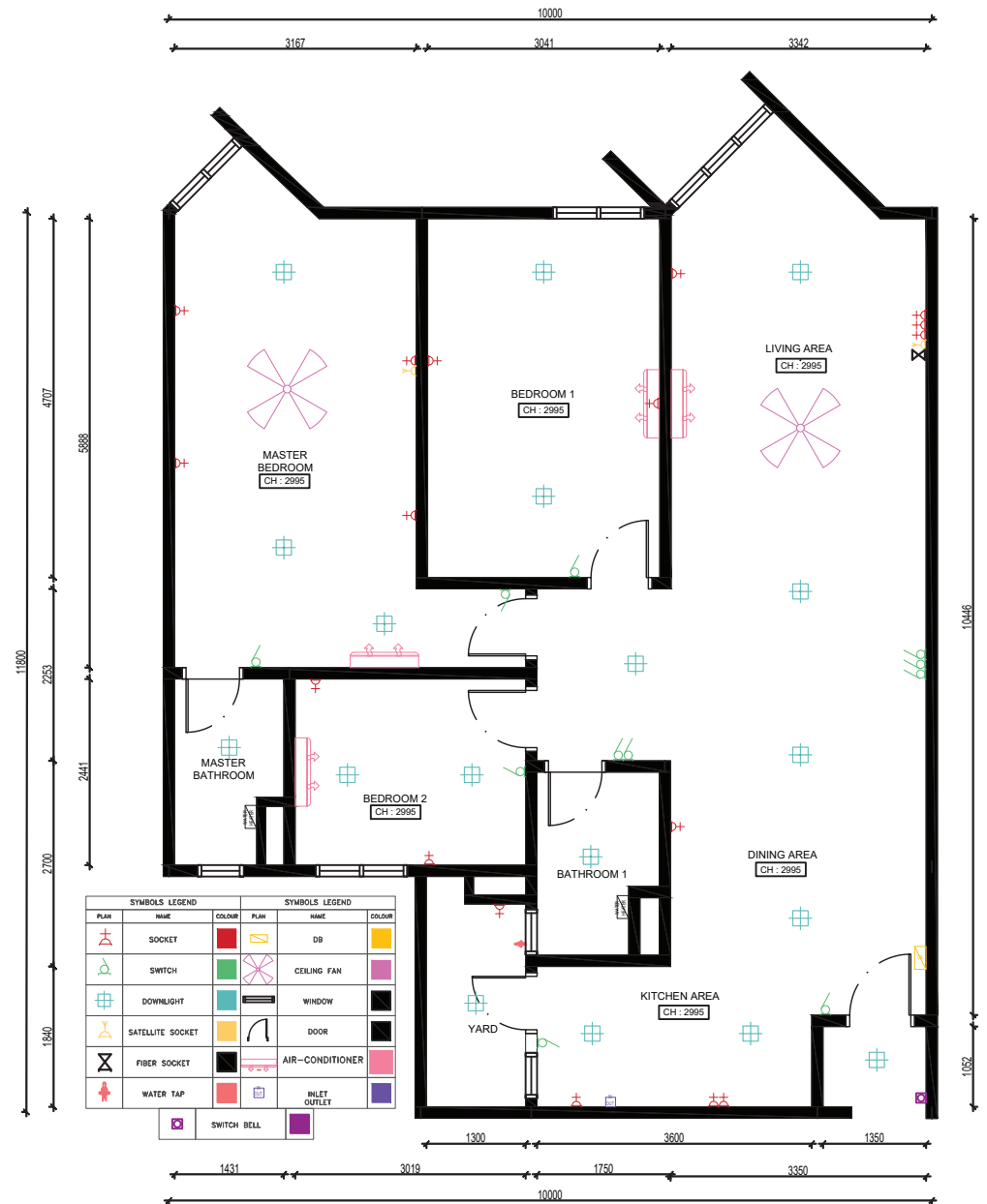
LAYOUT PLAN PLATINUM CASA DANAU RESIDENCE TYPE C1
