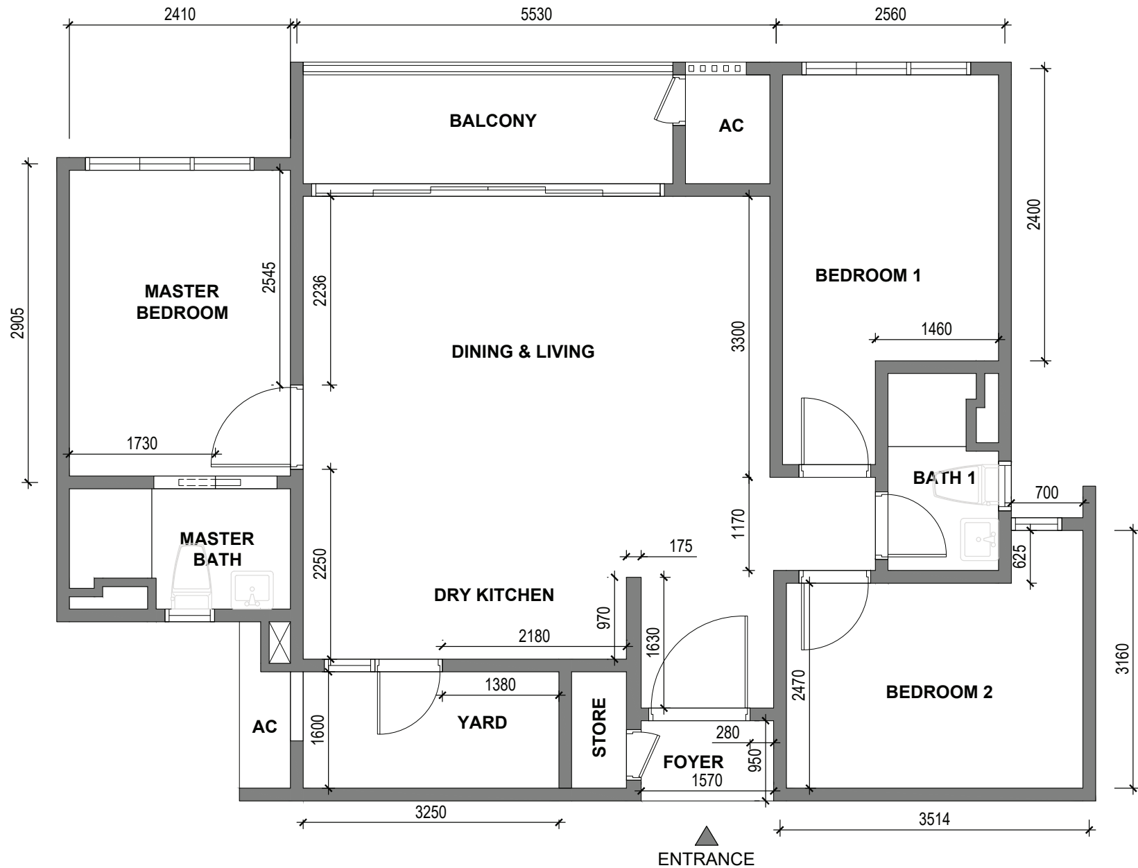
FURNITURE LAYOUT PLAN TYPE A
