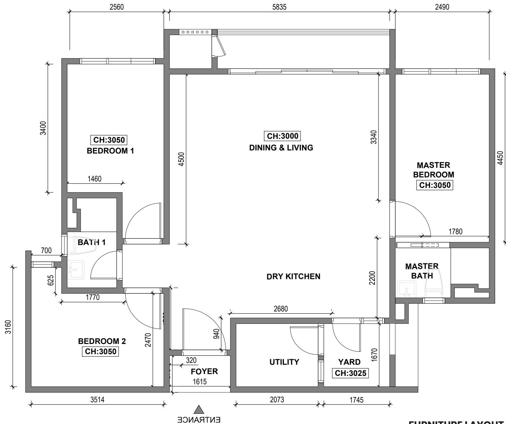
FURNITURE LAYOUT PLAN TYPE B
